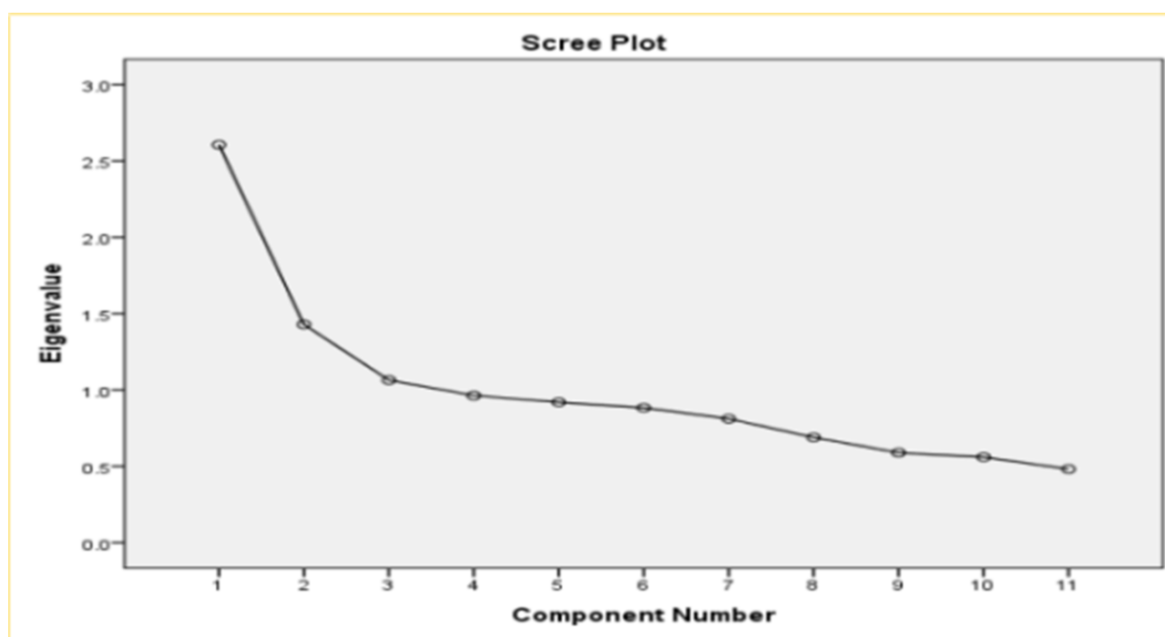
Figure 2. MPCK loading factor scree plot
