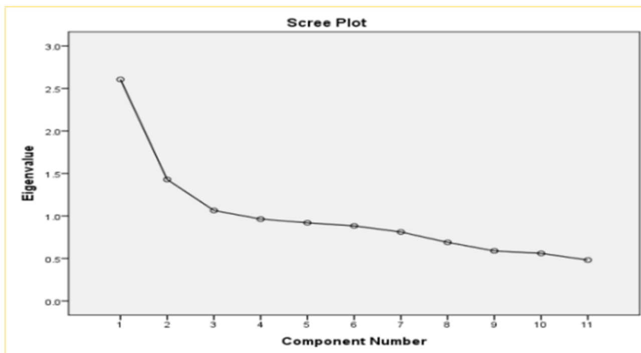
Figure 1. MCK loading factor scree plot
