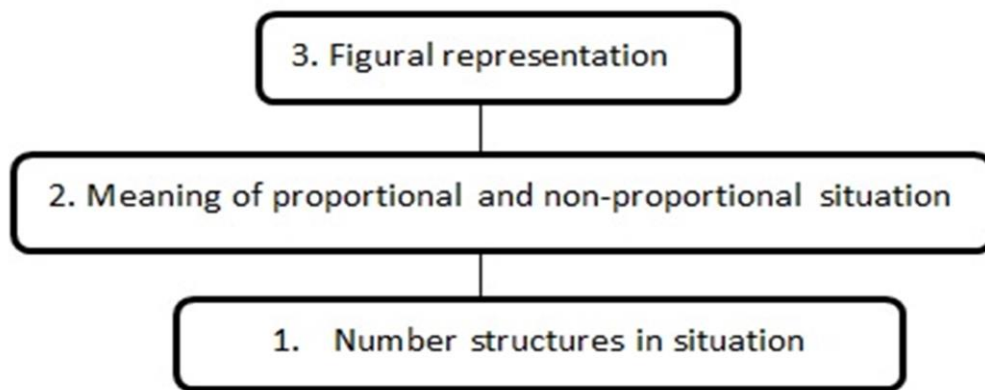
Figure 3. Hierarchical level of MCK of all teachers
