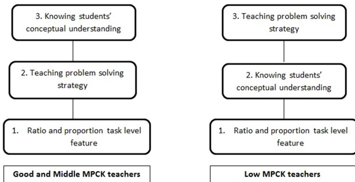
Figure 4. Hierarchical level of MPCK of teachers' assigned categories
